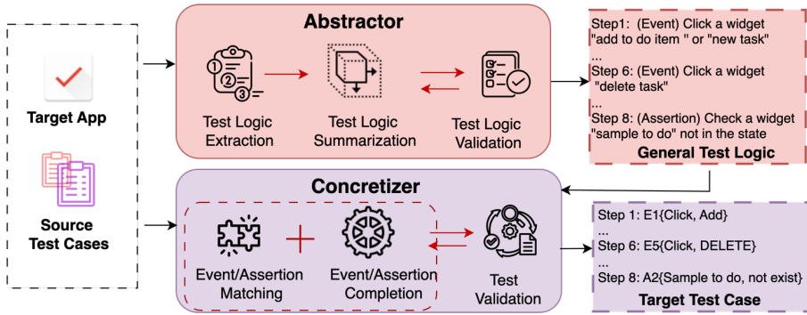
Fig. 2. Overview of MACdroid
